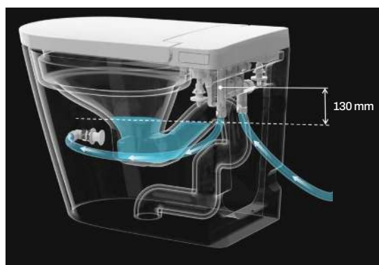
Anti-siphon open air gap
