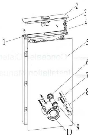
List of main installation accessories
